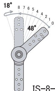
IS-8-132 zero position= 132° end position= 180°
