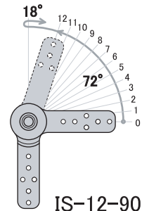
IS-12-90 zero position= 90° end position= 162°
