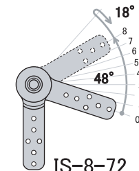
IS-8-72 zero position= 72° end position= 120°
