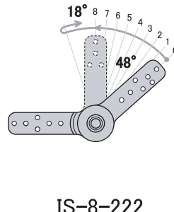
IS-8-222 zero position=222° end position= 270°
