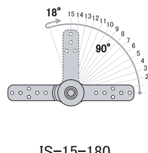
IS-15-180 zero position=180° end position= 270°
