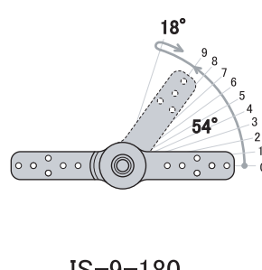
IS-9-180 zero position=180° end position= 234°
