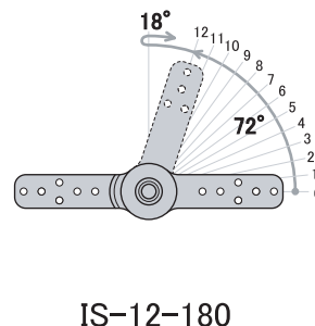
IS-12-180 zero position=180° end position= 252°
