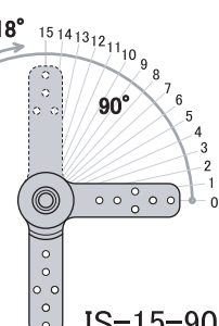
IS-15-90 zero position= 90° end position= 180°
